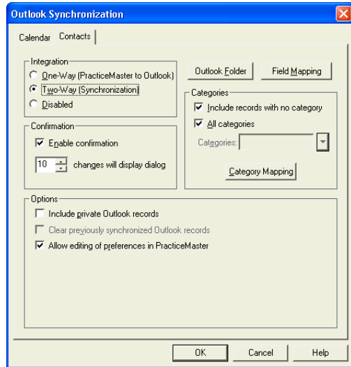
Figure 13, Version 15 Contacts tab
