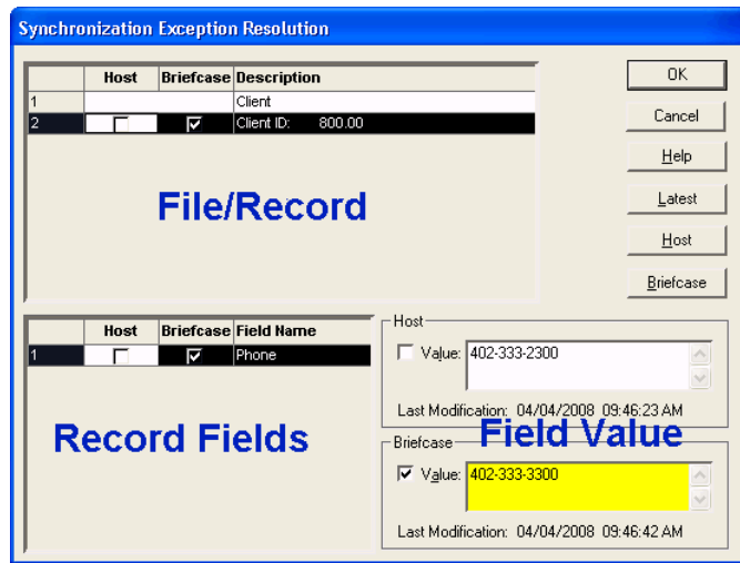
Fig. 5, Synchronization Exception Resolution for a single field
